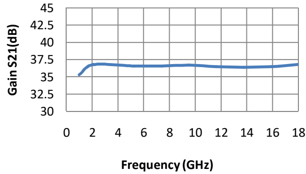
Gain S21
