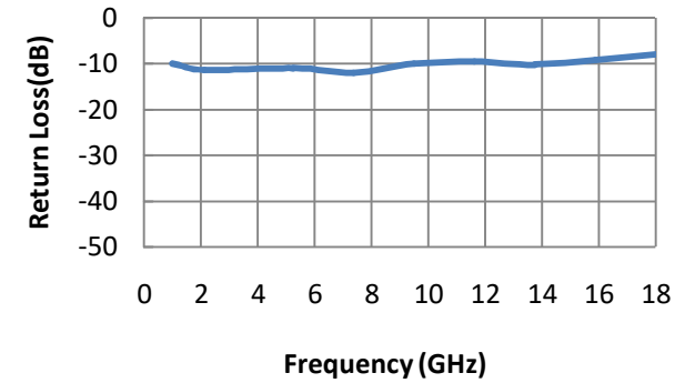
S11
