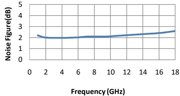
Noise Figure
