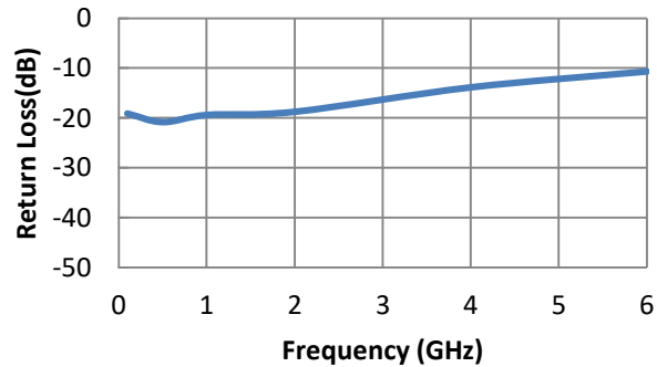
S22
