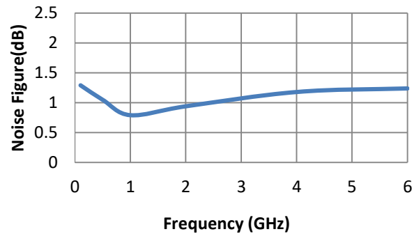
Noise Figure
